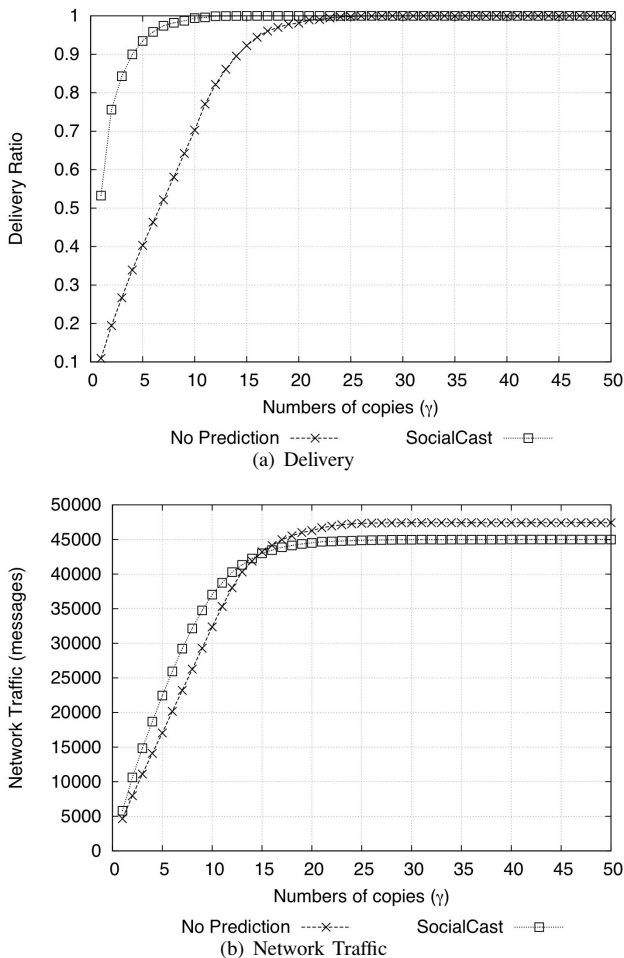
Fig. 3. Delivery and overhead against number of replicas.
