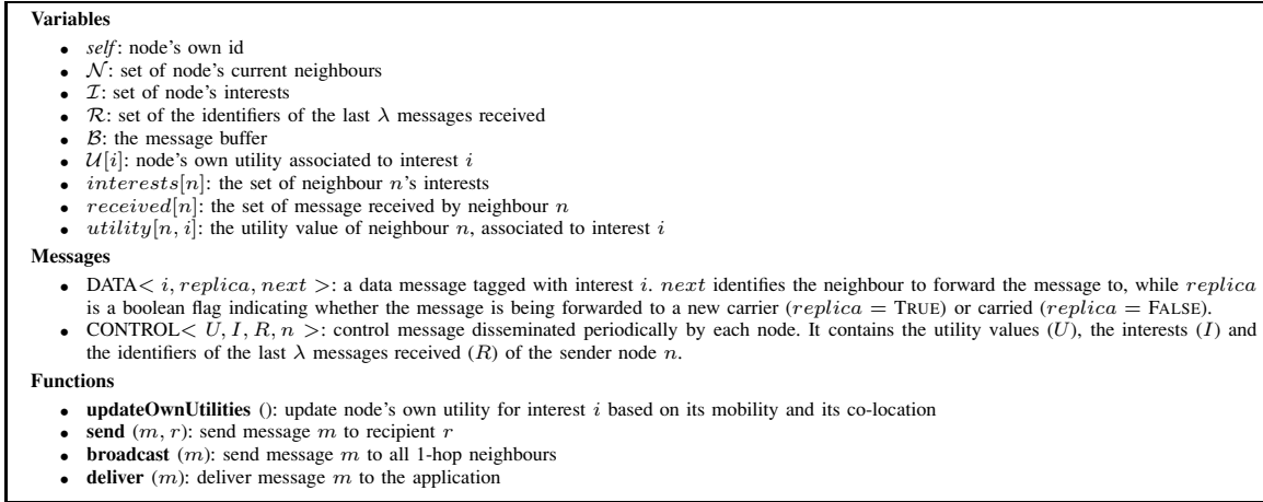
Fig. 1. Pseudo-code definitions of the SocialCast routing protocol.
