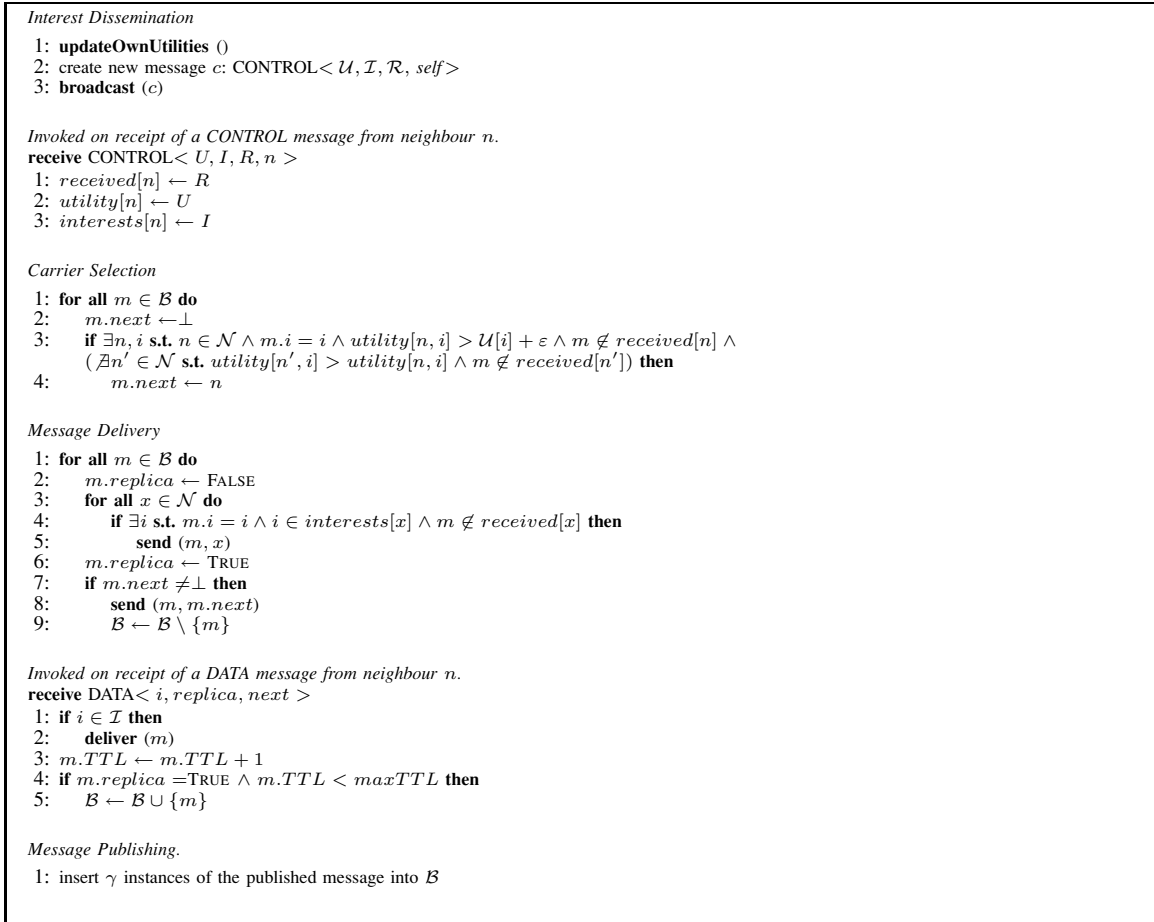
Fig. 2. Pseudo-code of the SocialCast routing protocol.
