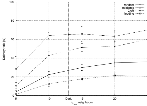
Figure 16: Impact of the structure of the potential contacts network (maximum number of neighbours): delivery ratio vs maximum number of neighbours.
