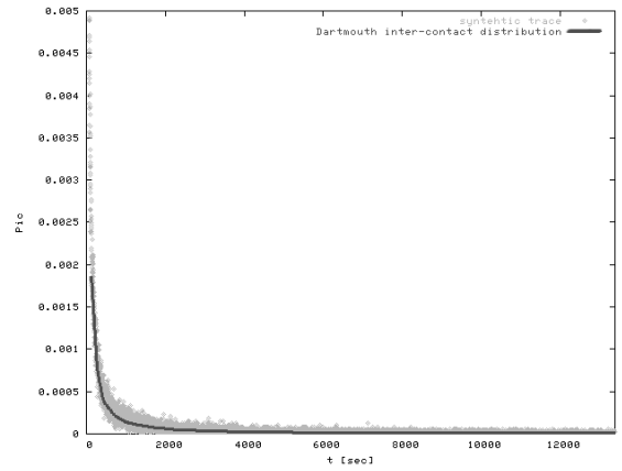
Figure 8: Comparison between synthetic trace and real power-law distribution using Dartmouth coefficient: inter-contact time.
