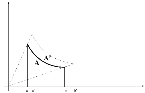
Figure 19: Scaling up (or down) a graph.
